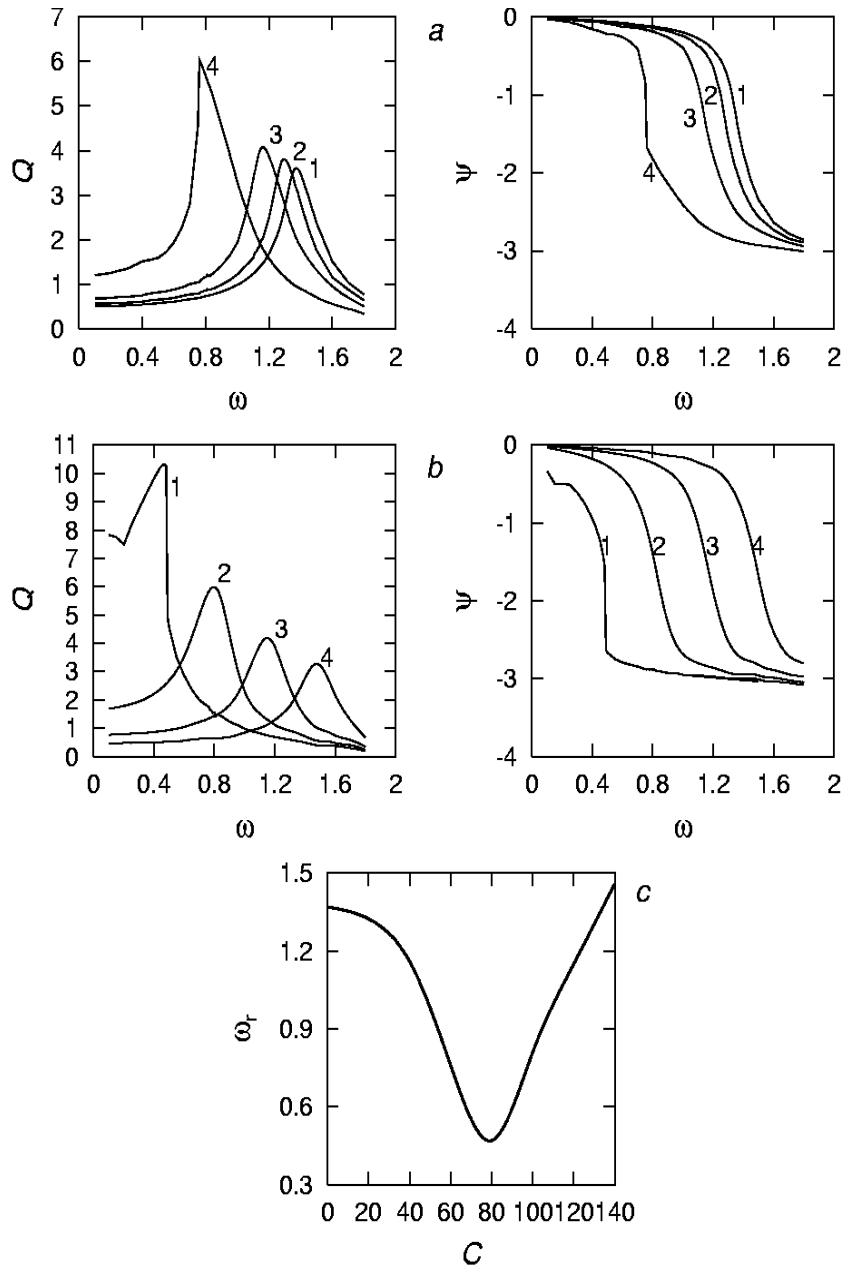
Figure 3. Dependences of the response amplitude Q and phase shift \psi on \omega for \delta = 0.1, \Omega = 9.842, A = 0.05 : (a) for vibration amplitudes C = 0, C = 25, C = 40 and C = 60 (curves 1, 2, 3 and 4, respectively); (b) for C = 80, C = 100, C = 120 and C = 140 (curves 1, 2, 3 and 4, respectively); (c) plot of the resonance frequency \omega_r as a function of C
