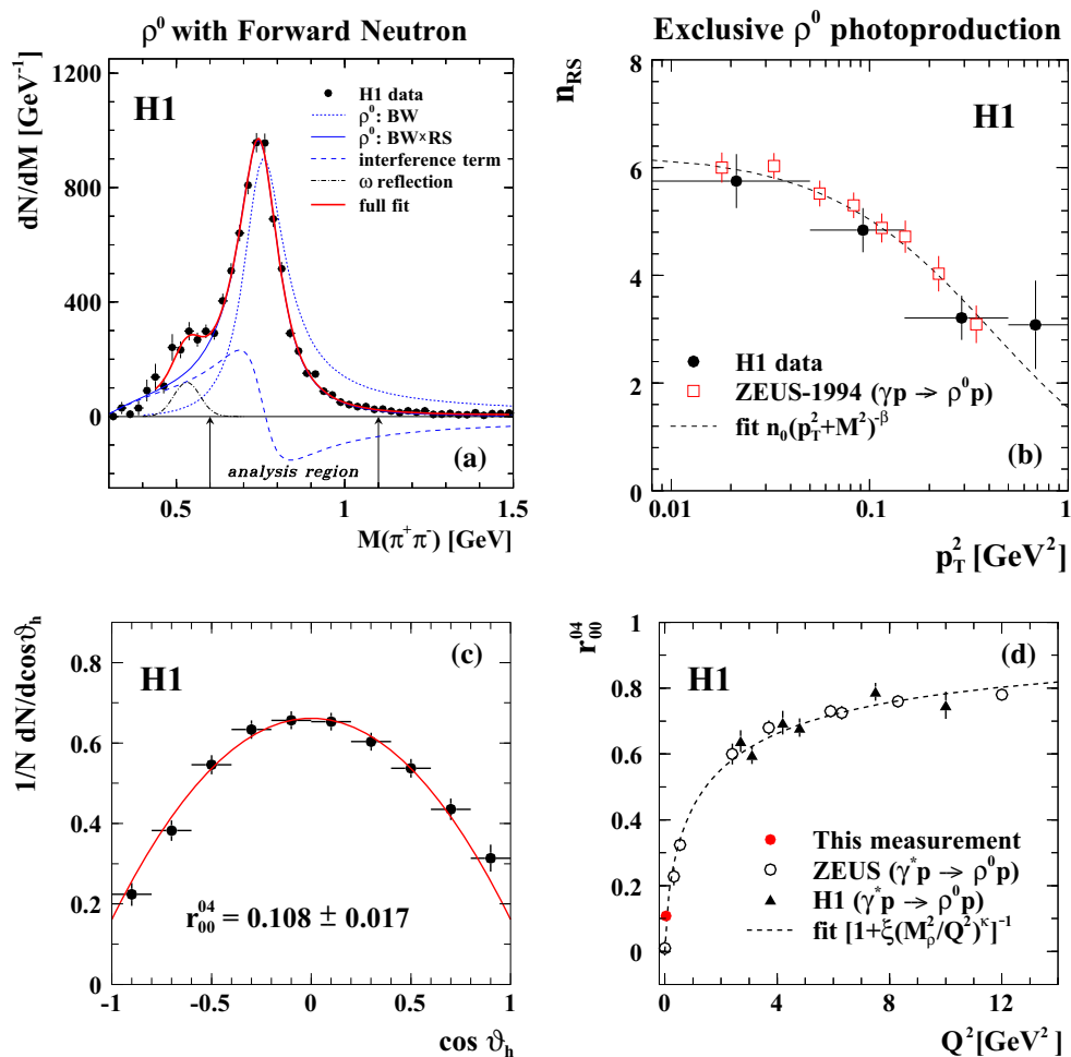
Fig. 3 The \rho^0 meson properties: a mass distribution of the \pi^+\pi^- system for exclusive \rho^0 production with p_T^2 < 1.0 GeV 2 associated with a leading neutron. The data points are corrected for the detector efficiency. The curves represent different components contributing to the measured distribution and the Breit–Wigner resonant part extracted from the fit to the data. The analysis region 0.6 < M_{\pi^+\pi^-} < 1.1 GeV is indicated by vertical arrows. b Ross–Stodolsky skewing parameter,
