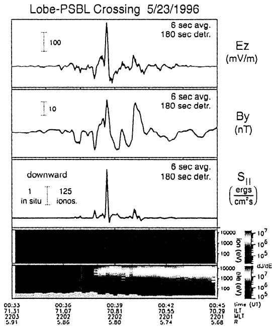
Figure 1. Measurements from the Polar satellite on 5/23/1996 during a lobe-PSBL crossing. The panels show, from top to bottom, the electric field component approximately normal to the plane of the plasma sheet boundary, the east-west component of the magnetic field (model subtracted), the Poynting flux component along the magnetic field, and energy-time spectrograms of ions and electrons.
