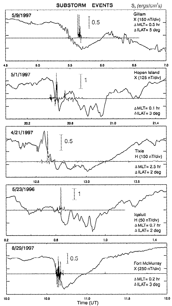
Figure 3. Temporal comparison of in-situ field-aligned Poynting flux (red line) measured by Polar and ground signatures of H-bays (black lines). The Poynting flux component shown is parallel to the average background magnetic field. The Poynting flux scale shows in situ values. Positive values indicate directions downward, towards the ionosphere. The relative separation between Polar's footpoint and the ground stations is given as \Delta MLT and \Delta ILAT.
