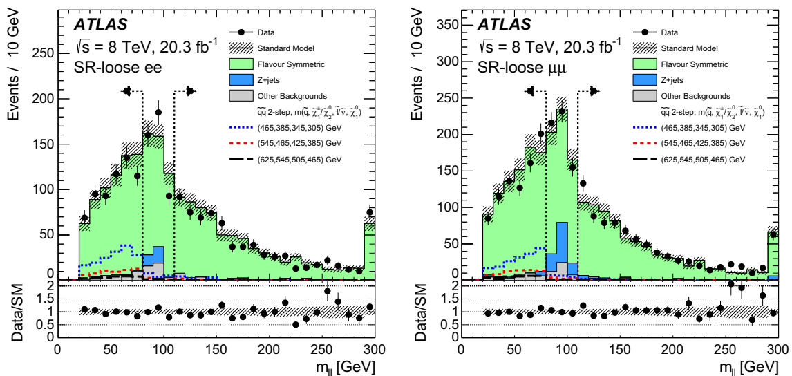
Fig. 9 (Corrected version): The observed and expected dilepton mass distributions in the off-Z SR-loose. The vertical dashed lines indicate the 80 < m_{\ell\ell} < 110 \text{ GeV} region, which is used to normalise the Z + jets background and is thus not treated as a search region. Example
