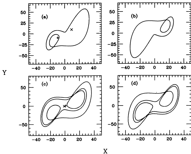
FIG. 2. Plots (a) and (b) show the computed x - y projections of the pair of Lorenz periodic attractors for r = 100.00 . The cross and plus symbols in (a) and (b) indicate the positions of the centers of mass for (a) and (b), respectively, which differ significantly from each other. Plots (c) and (d) provide the corresponding information for the pair of attractors at r = 126.49 ; note that their centers of mass are almost coincident.
