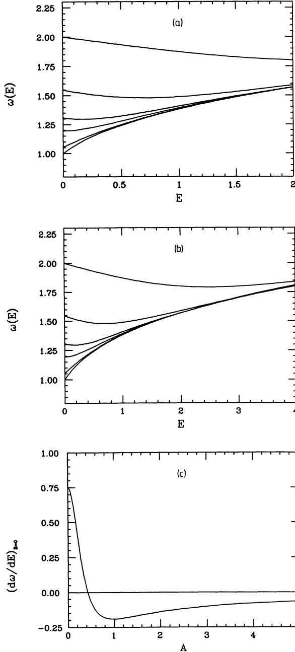
FIG. 1. (a) The dependence of the eigenfrequency \omega(E) of the oscillations on the energy E of the oscillator, measured from the bottom of the potential well, for several values of the inclination parameter A , calculated from Eqs. (4a) and (4b). The corresponding values of A , from bottom to top, were 0, 0.2, 0.43, 0.6, 1.0 and 2.0. (b) As in (a), but over a wider range of E . (c) The dependence on A of the initial gradient \omega'_0 = [d\omega(E)/dE]_{E=0} of the curves shown in (a), calculated from (5) and (6).
