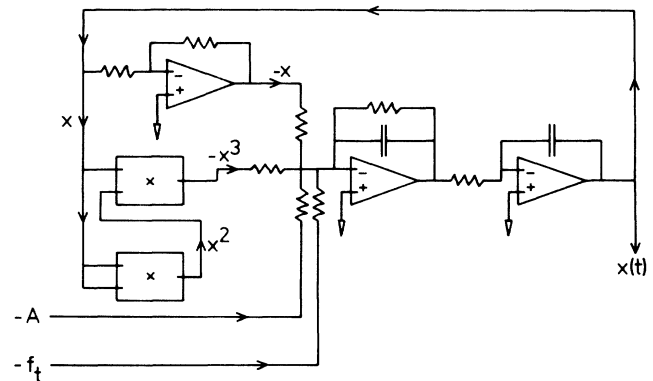
FIG. 5. Block diagram of the circuit used to model the system (2) and (7).
