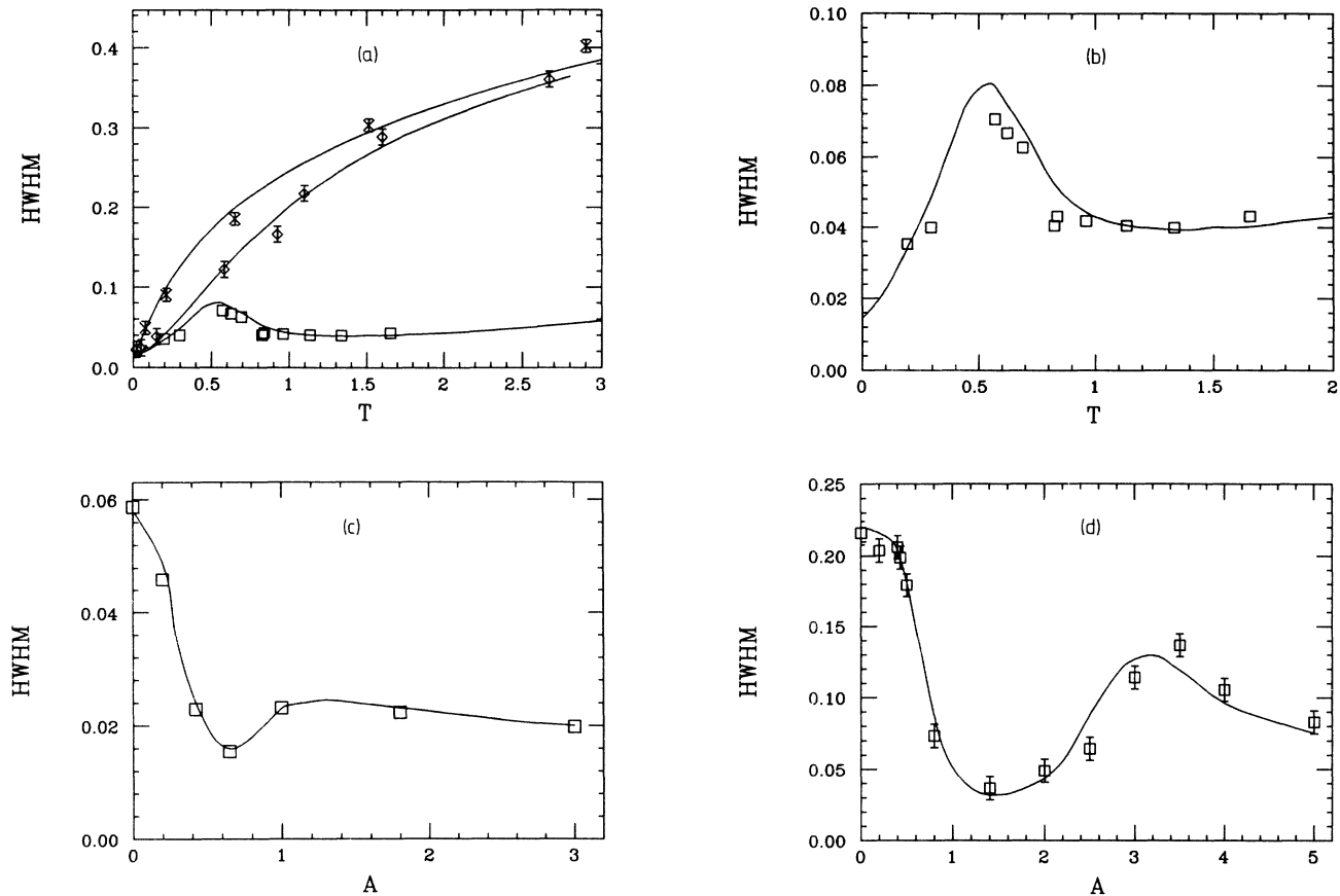
FIG. 6. The spectral width, defined as the half width at half maximum (HWHM), \delta\Omega , of the spectral peaks of the system (2) and (7) measured (data points) for the analog electronic model and calculated (solid curves) from (16) under different conditions. (a) Spectral width HWHM as a function of noise intensity T for three values of the inclination parameter: A=0 ( \times ); 0.43 ( \diamond ); 2.0 ( \square ). (b) As in (a), but plotted with an expanded ordinate scale for A=2.0 to demonstrate more clearly the spectral narrowing phenomenon: there is a range of noise intensities T for which the HWHM markedly decreases with increasing T . (c) Spectral width, HWHM, as a function of the inclination parameter A for a noise intensity T=0.098 . The experimental uncertainty is approximately the same size as the symbols. (d) Spectral width, HWHM, as a function of A for T=0.98 .
