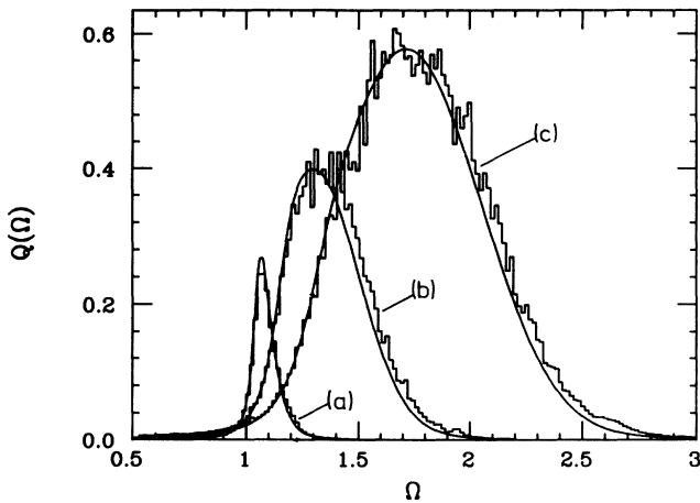
FIG. 2. Spectral density of the fluctuations Q(\Omega) of the oscillator (2) and (7) calculated (solid curves) from (16) and measured (histograms) for the analog electronic model, with the inclination parameter A=0 , for noise intensities: (a) T=0.078 ; (b) 0.687 ; (c) 3.04 .
