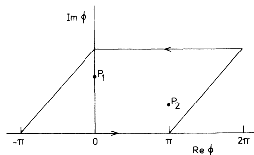
FIG. 7. Contour of integration for the determination of the harmonics of the coordinate.
