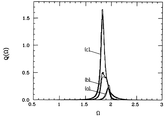
FIG. 4. Spectral density of the fluctuations Q(\Omega) of the oscillator (2) and (7) calculated (solid curves) from (16) and measured (histograms) for the analog electronic model with the inclination parameter A=2.0 , for noise intensities: (a) T=0.078 ; (b) 0.687 ; (c) 3.04 .
