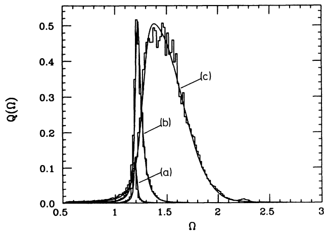
FIG. 3. Spectral density of the fluctuations Q(\Omega) of the oscillator (2) and (7) calculated (solid curves) from (16) and measured (histograms) for the analog electronic model with the inclination parameter A=0.43 for noise intensities: (a) T=0.0191 ; (b) 0.154 ; (c) 1.15 .
