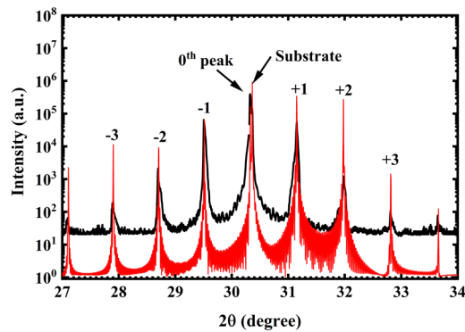
Fig. 1. HRXRD curve of InAs/InAsSb superlattice grown on GaSb substrate.
