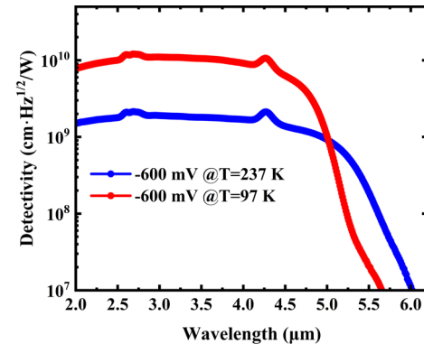
Fig. 5. Detectivity spectra of nBn InAs/InAsSb device at 97 K and 237 K.
