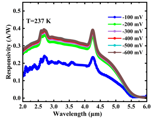
Fig. 4. Photo response varies as reverse bias voltage spectra at T=237 \text{ K} .
