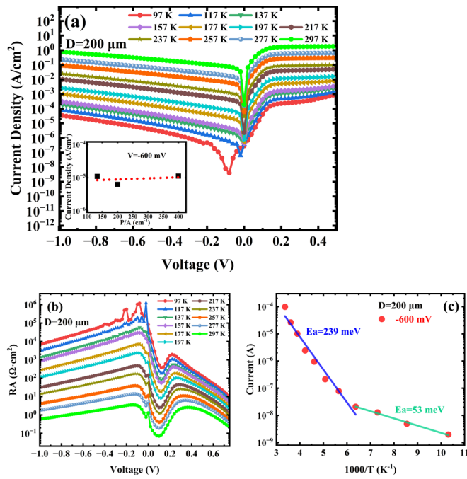
Fig. 3. Temperature dependent (a) dark current and (b) RA characteristic of 200 \mu\text{m} diameter InAs/ InAsSb nBn device. The inset of Fig. 3(a) is the dark current density as a function of perimeter to area ratio (P/A). (c) Arrhenius plot of 200 \mu\text{m} diameter InAs/ InAsSb nBn device under reverse bias of -600 mV.
