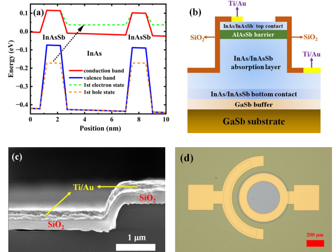
Fig. 2. (a) Band diagram of InAs/InAsSb superlattice; (b) Schematic of fabricated InAs/InAsSb nBn device; (c) SEM image of passivated mesa side wall of the device; (d) Microscope image of the InAs/InAsSb nBn device.
