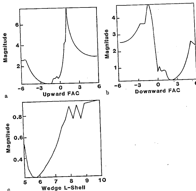
Fig. 4a-c. Model deviations projected onto each parameter axis for the Day 237, 1990 event. For values along the x-axis of each graph the minimum deviation between model and data was evaluated through optimisation of the other two parameters alone
