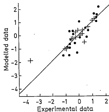
Fig. 21. Comparison between modelled zero field deviations and high-latitude SAMNET data. The circles represent the H -component, and the crosses the D -component. The least squares gradient is 0.97
