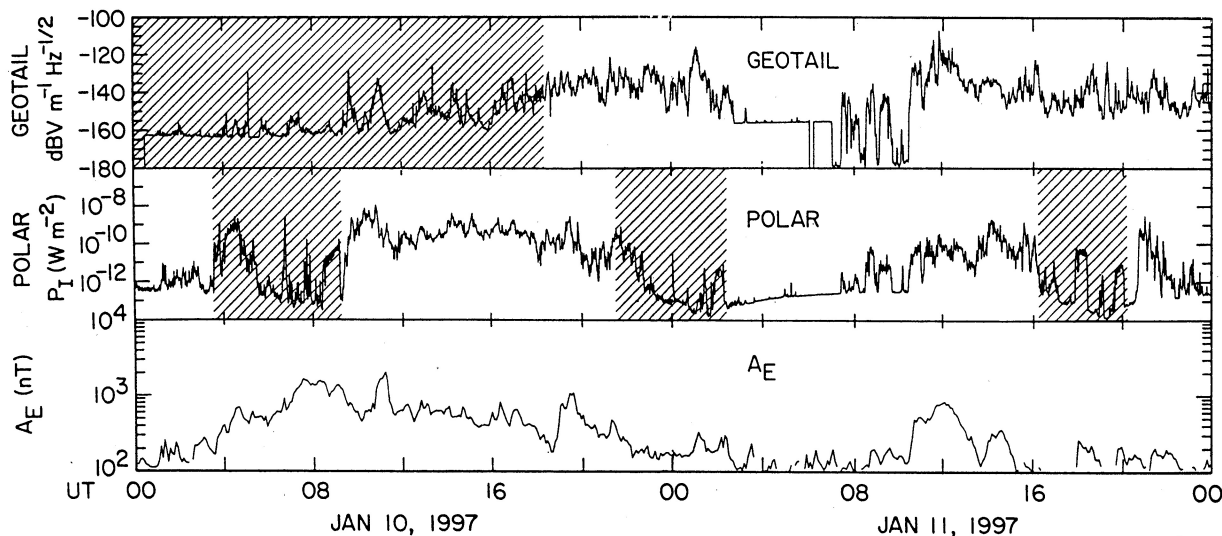
Figure 2. The auroral electrojet index (bottom), integrated AKR power flux from Polar (middle) and the Geotail AKR index for the January 10-11 interval. The hatched regions represent times when one of the spacecraft is outside of the nominal 178-kHz emission cone and when the integrated power flux is not expected to accurately represent AKR activity, in general.
